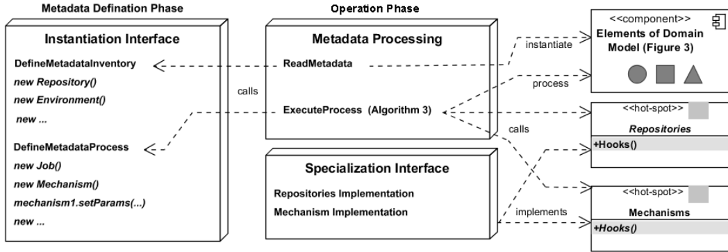
Fig. 5. Overview of FramETL framework
